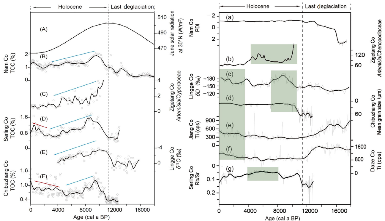
Fig. 1. The environmental changes since last deglaciation period reflected by lakes cores of Lingge Co, Serling Co and Chibuzhang Co together with other literatures. The left part shows variations in temperature, with blue arrows showing the cooling trend and red arrows indicating the warming trend. (A) Solar radiation changes at 30°N [9]. (B) TOC record from Nam Co [10]. (C) Pollen ratio of Artemisia/Cyperaceae in pollen assemblages from Lake Zigetang [11]. (D) TOC record from Serling Co [8]. (E) \delta^{18}\text{O} record of Leucocythere mirabilis shells from Lingge Co [12]. (F) TOC record from Chibuzhang Co. The right part shows the variations in moisture (or precipitation) and green shadows indicate relatively humid periods. (a) Pollen discrimination index (PDI) record from Nam Co [10]. (b) Pollen ratio of Artemisia/Chenopodiaceae in pollen assemblages from Lake Zigetang [11]. (c) Weighted average \delta D values for \text{C}_{26} , \text{C}_{28} and \text{C}_{30} n -alkanoic acids from Lingge Co [13]. (d) Mean grain size record of Chibuzhang Co. (e) Ti record from Jiang Co [14]. (f) Ti record from Daze Co [14]. (g) Rb/Sr record from Serling Co [8].
